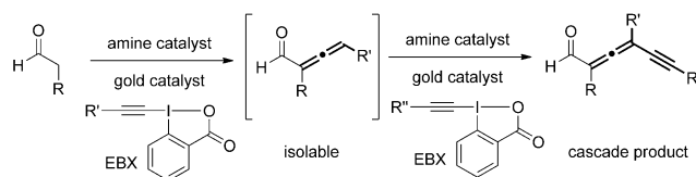
Scheme 1. \alpha -Functionalization of aldehydes by enamine/metal synergistic catalysis.
